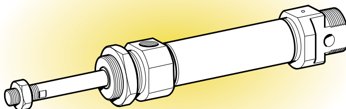
Single-acting, spring-extended
