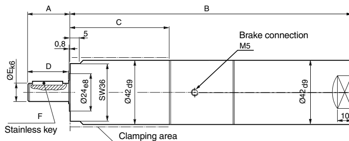
P1V-S030A with shaft with keyed shaft
