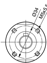
P1V-S030D with threaded shaft
